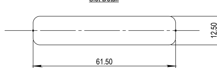
Slot Detail
